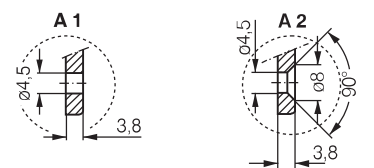
Barbed inserts
